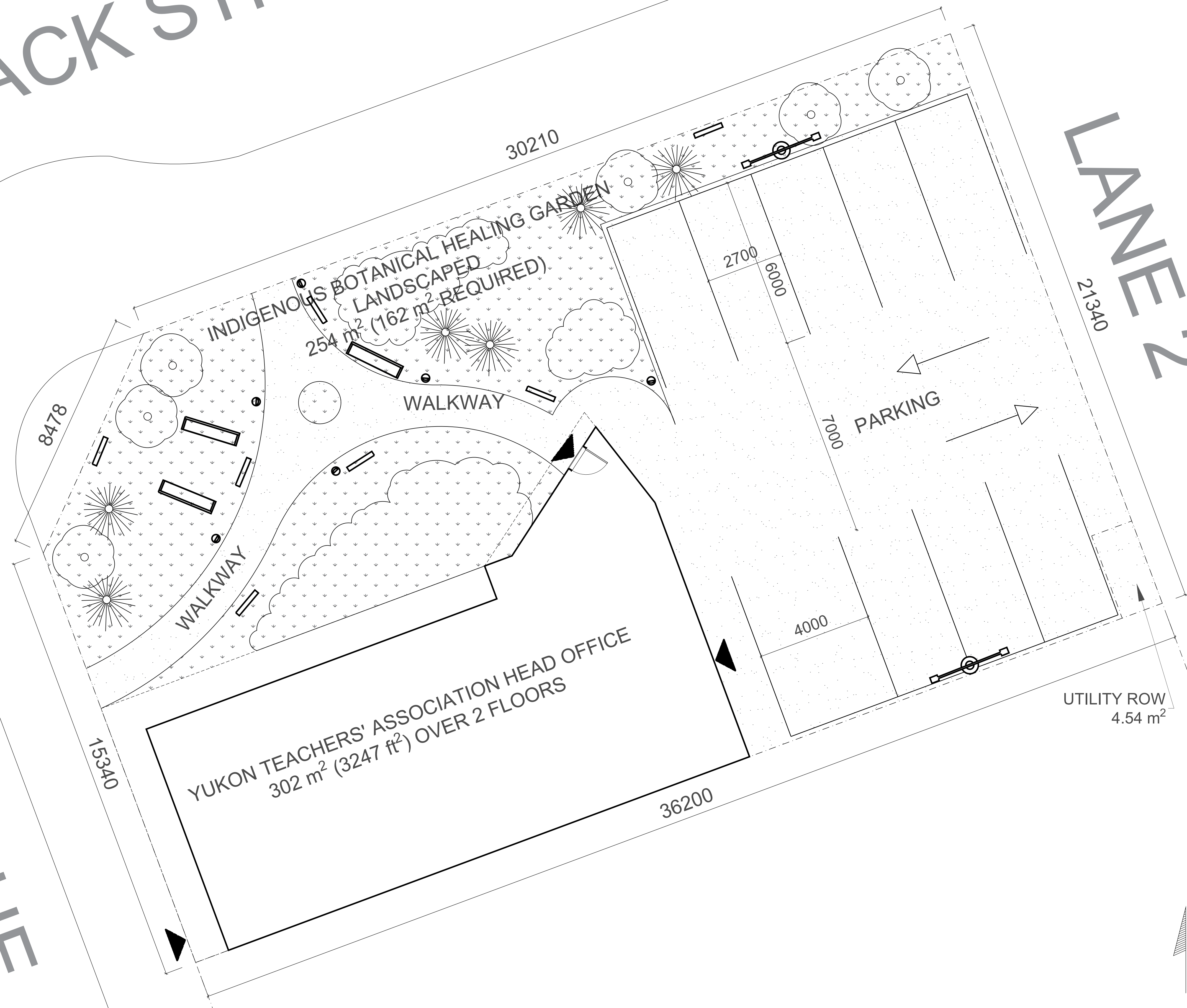
1 LANDSCAPE PLAN A001 1:100
